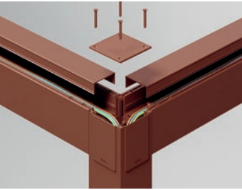
Easy access in-wall wiring
